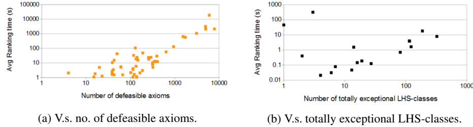
Fig. 3: Ranking computation performance (ranking time).
