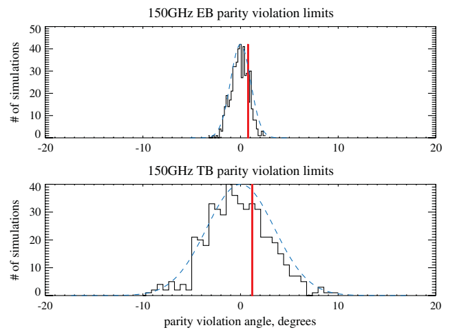
FIG. 1 (color). \Delta\alpha measured from QUaD 150 GHz TB and EB spectra; histogram of simulations and red line for data. The histogram does not account for systematic error. The dotted line indicates total uncertainty assuming a Gaussian 0.5^\circ systematic error.
