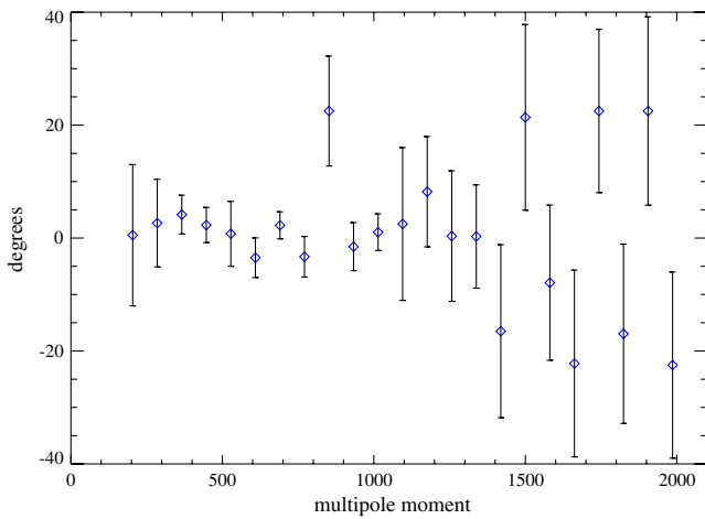
FIG. 2 (color online). 150 GHz \Delta\alpha per-band power derived from the EB spectrum. Note that in practice these points are combined before the final transformation to \Delta\alpha —the purpose of this plot is to give a visual representation of the relative uncertainties across the band powers.
